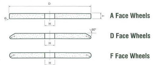
Type 1 (Straight Wheels)
